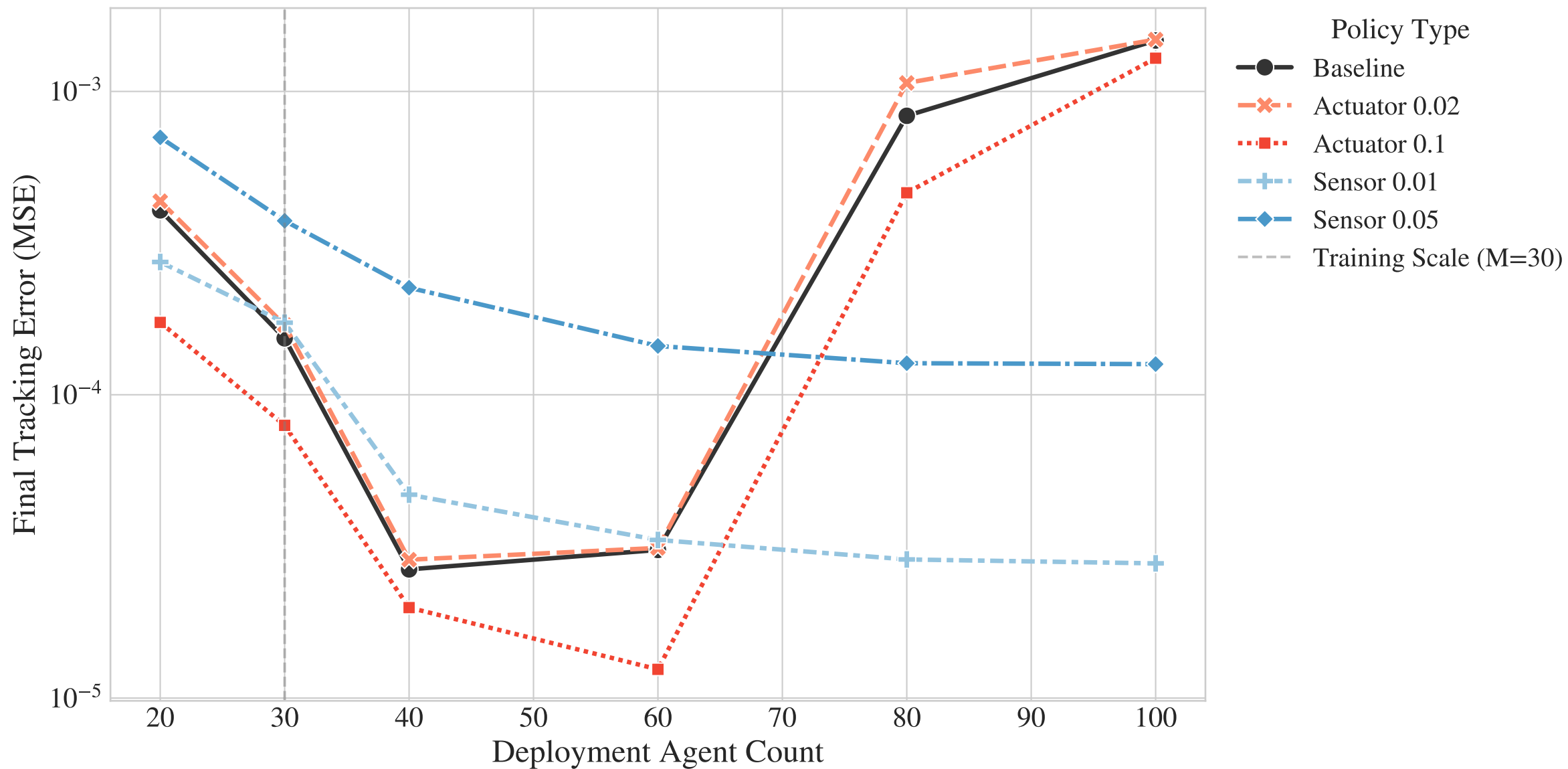
Robustness in Actuator Mid Env ( \sigma_u = 0.1, \sigma_z = 0.0 )
