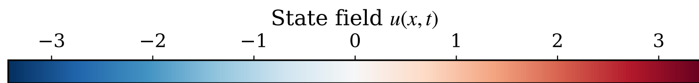
Natural Evolution (L=64)
