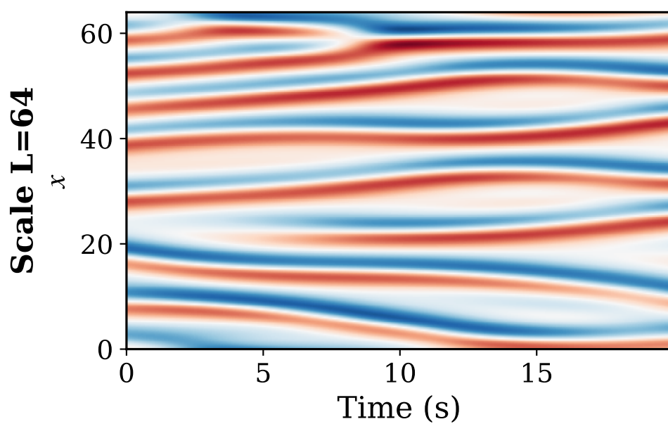
Natural Evolution (L=64)
