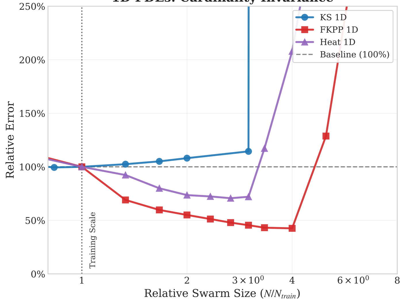
1D PDEs: Cardinality Invariance
