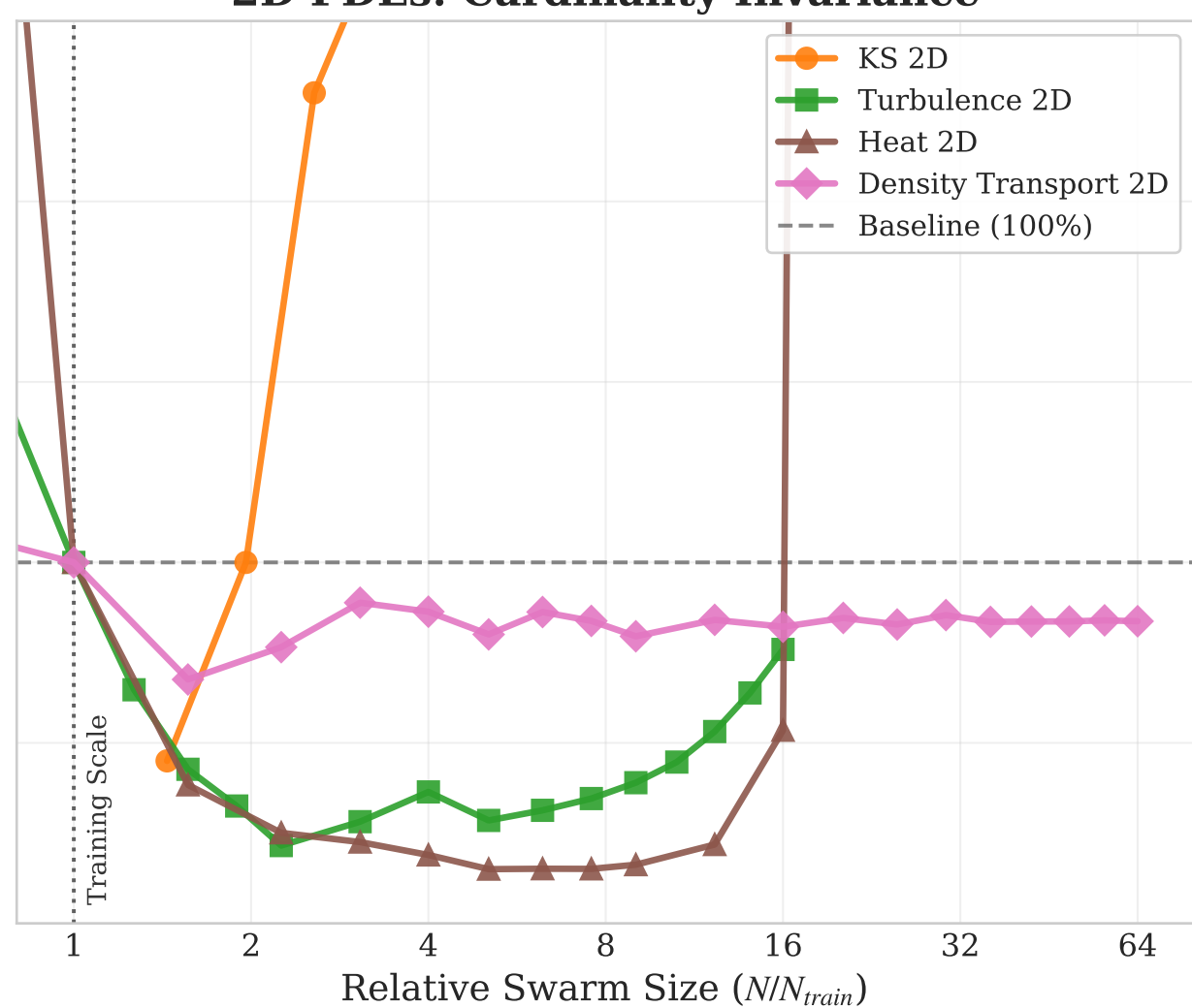
2D PDEs: Cardinality Invariance
