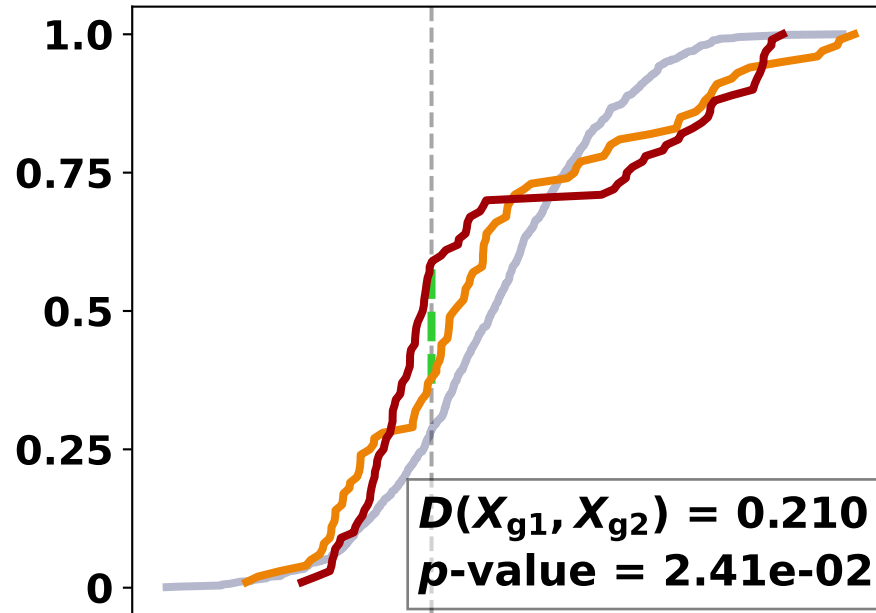
KS Statistic
