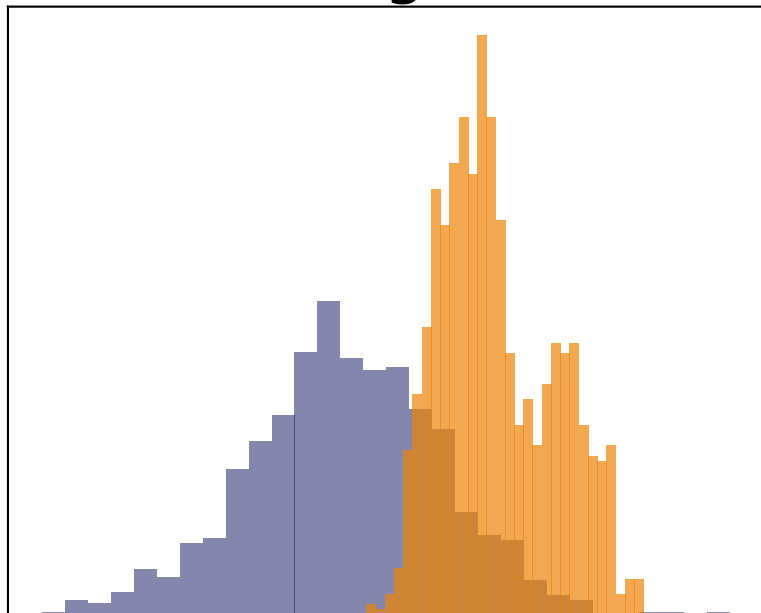
Histogram
