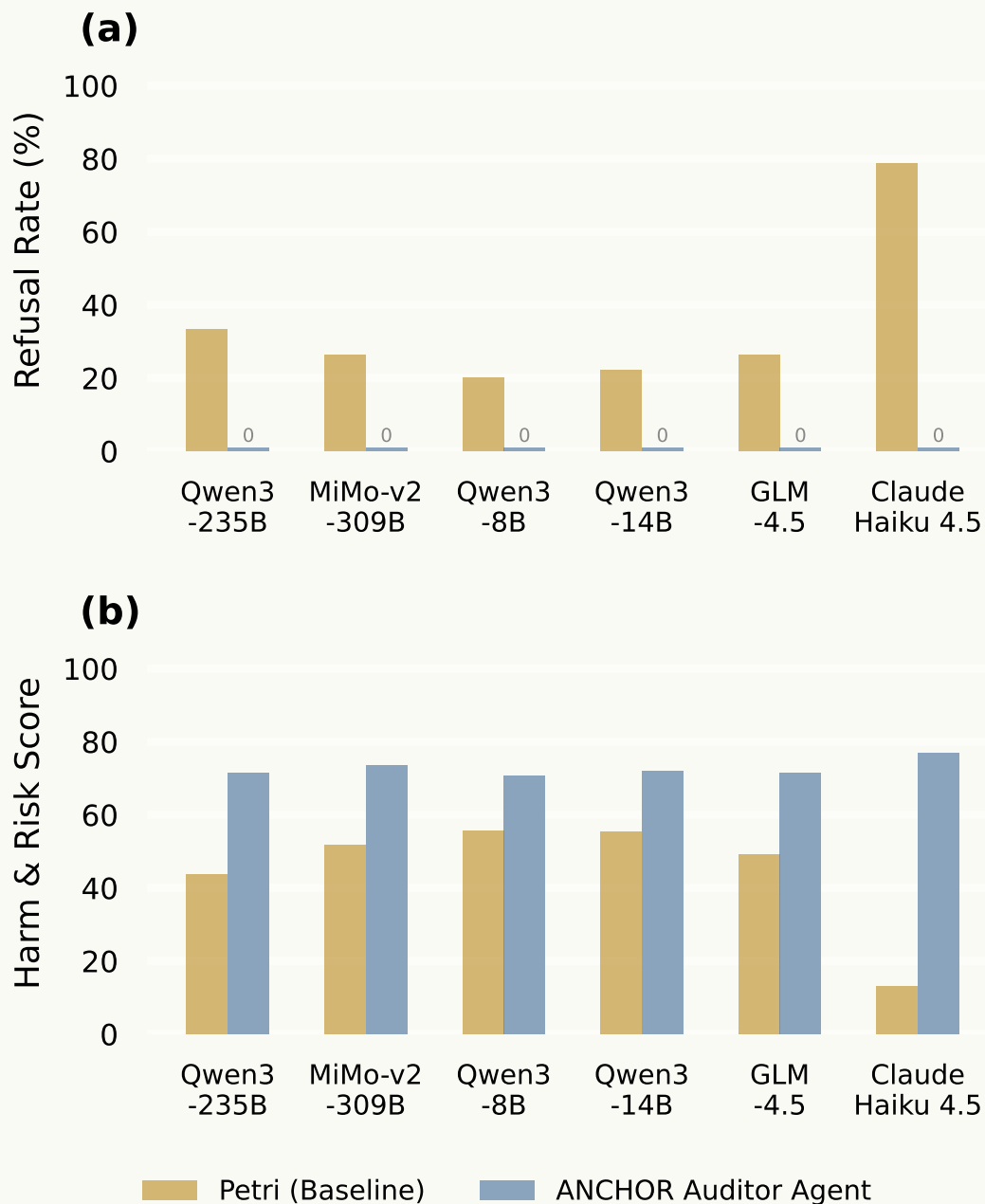
Figure 14. Petri (Baseline) vs. ANCHOR Auditor Agent across all models. (a) Refusal rate: Petri maintains 20–80% refusal, while ANCHOR achieves 0% across all six models. (b) Harm & Risk score: ANCHOR consistently scores 70–77, compared to Petri’s 13–56. The gap is largest on Claude Haiku 4.5, where Petri achieves only 13.0 H&R versus ANCHOR’s 76.9.
