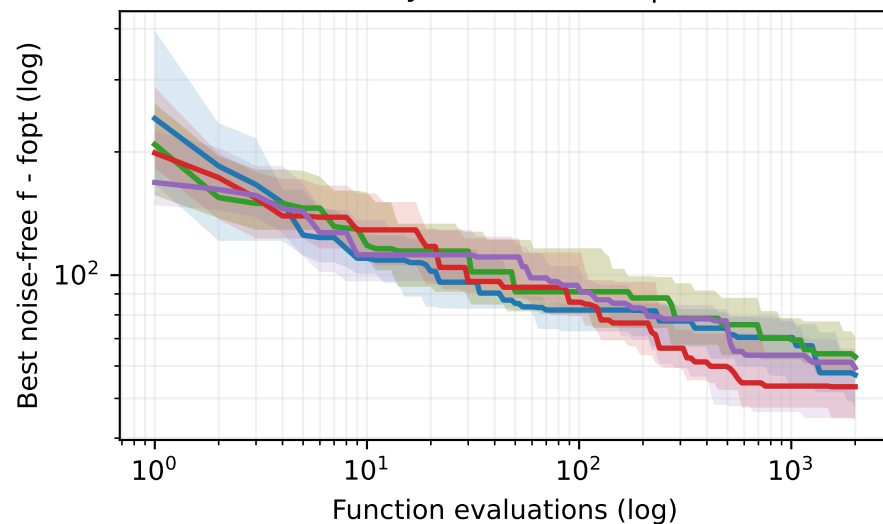
bbob-noisy f20 (id=120) | D=40
