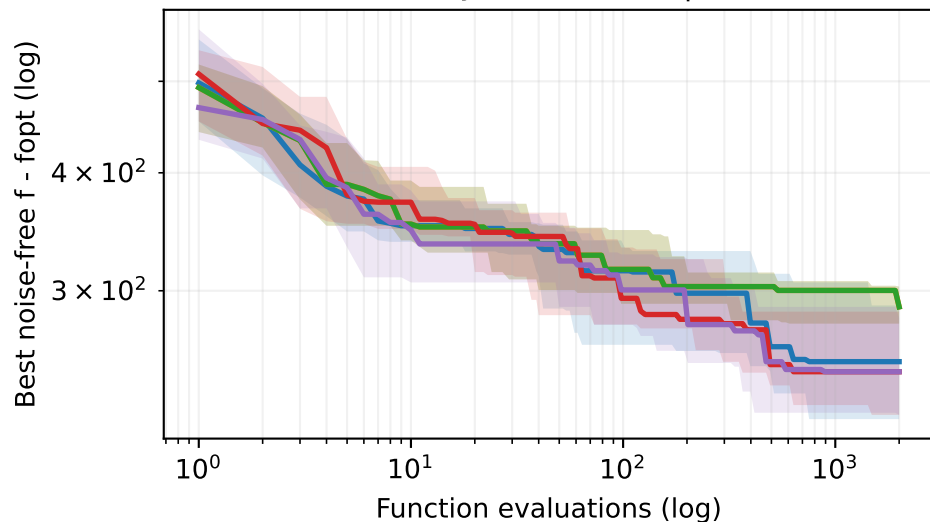
bbob-noisy f8 (id=108) | D=40
