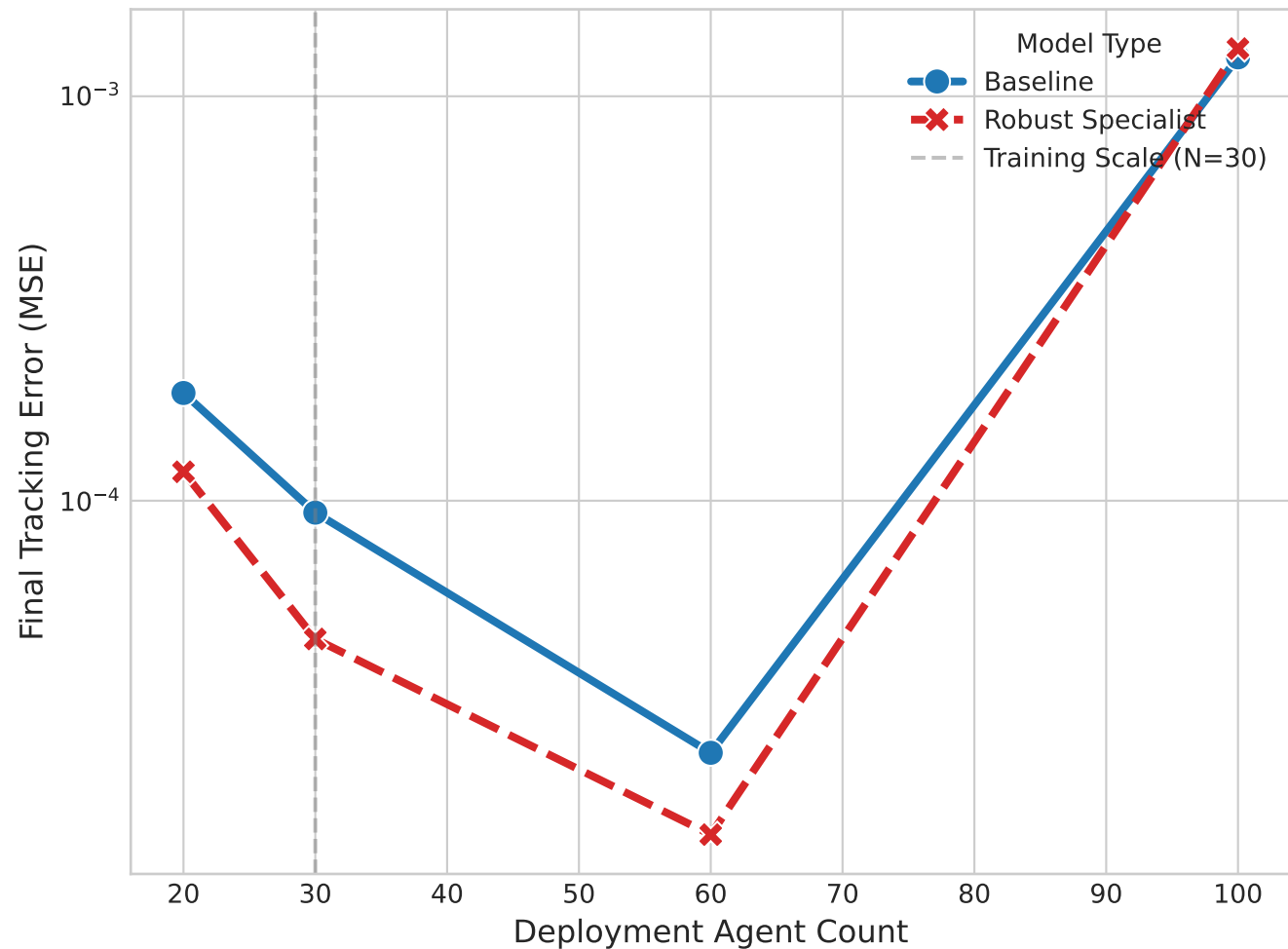
Robustness to Execution Errors (Actuator Noise \sigma_u = 0.5 )
