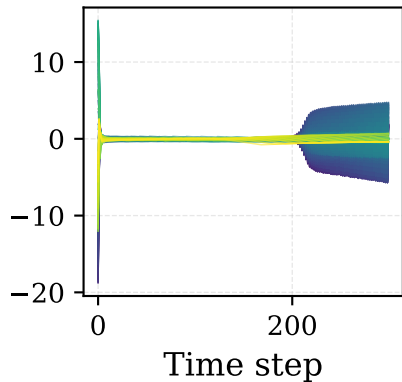
Control u_i(t)
