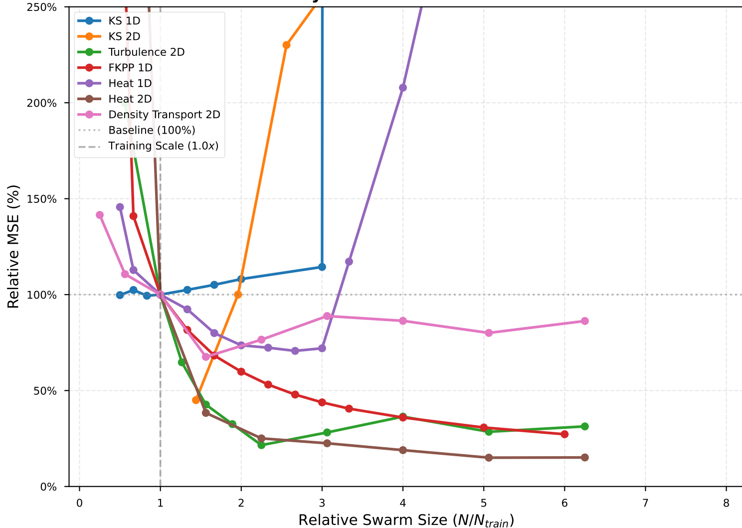
Zero-Shot Scalability: Relative MSE vs Relative Swarm Size
