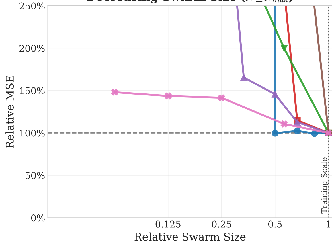
Decreasing Swarm Size ( N \leq N_{train} )
