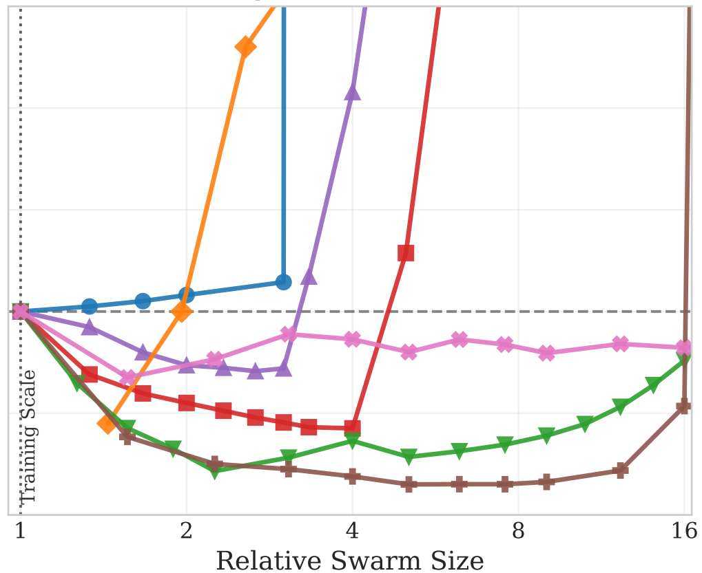
Increasing Swarm Size ( N \geq N_{train} )
