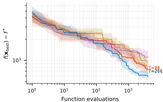
bbob-noisy f25
