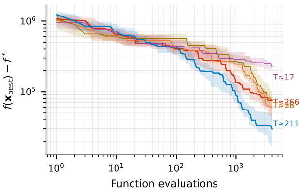
bbob-noisy f16
