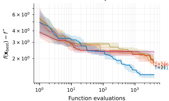
bbob-noisy f25
