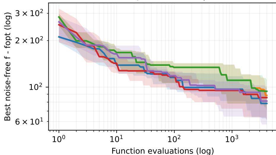
bbob-noisy f8 (id=108) | D=20
