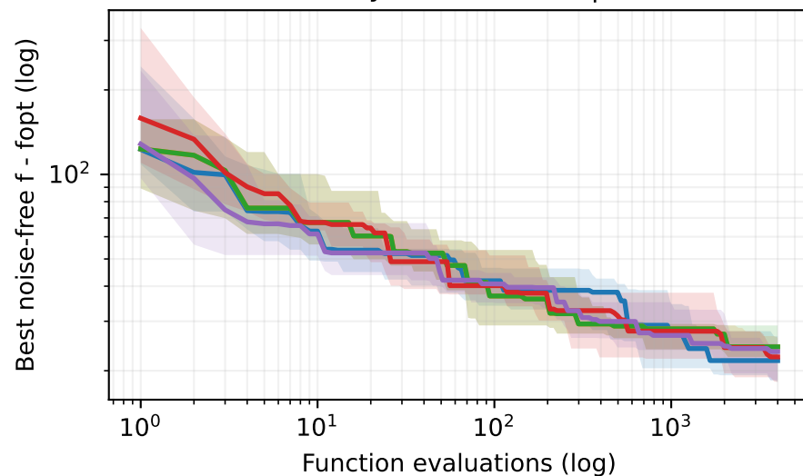
bbob-noisy f20 (id=120) | D=20
