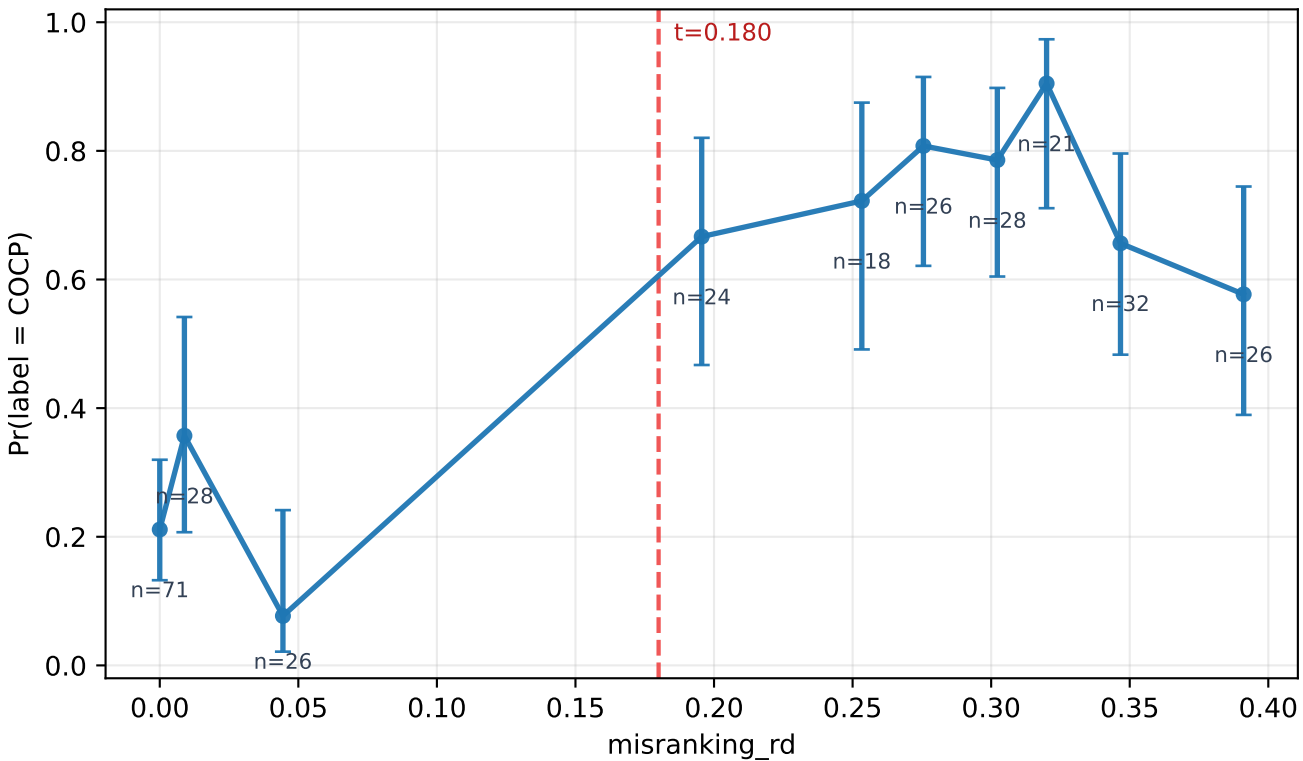
bbob-noisy D=40, B=200D: calibration (test split)
