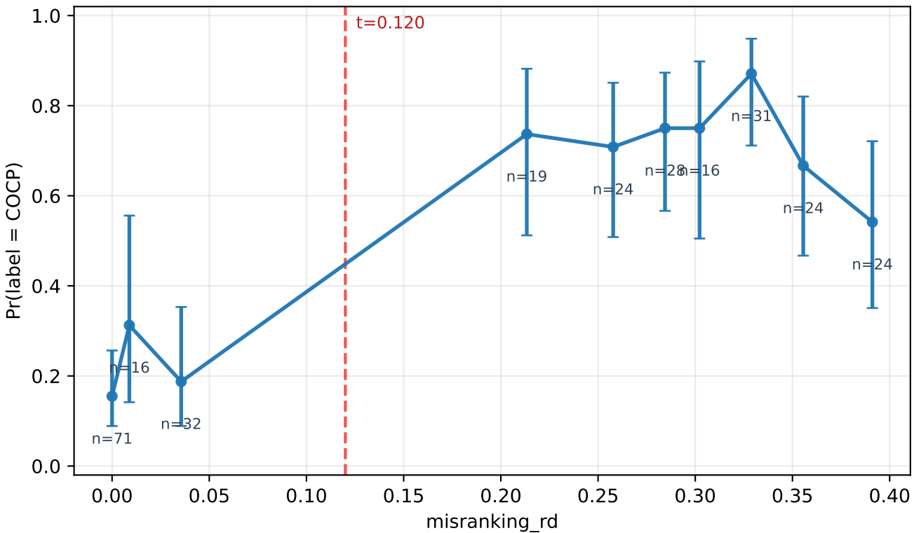
bbob-noisy D=40, B=500D: calibration (test split)
