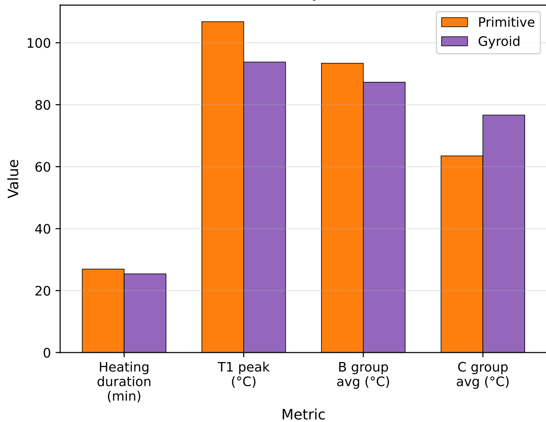
Primitive vs Gyroid (10W)
