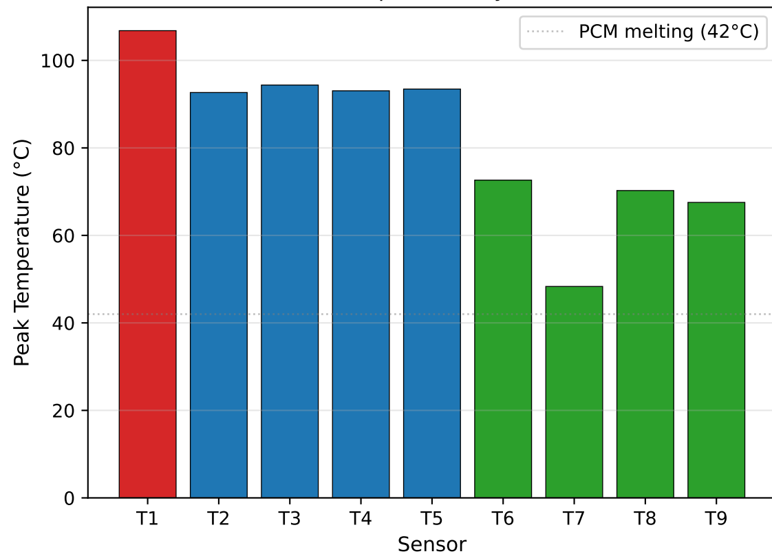
Peak Temperature by Sensor
