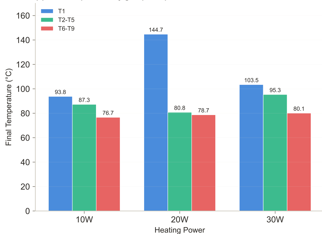
(a) Final temperature by group and power
