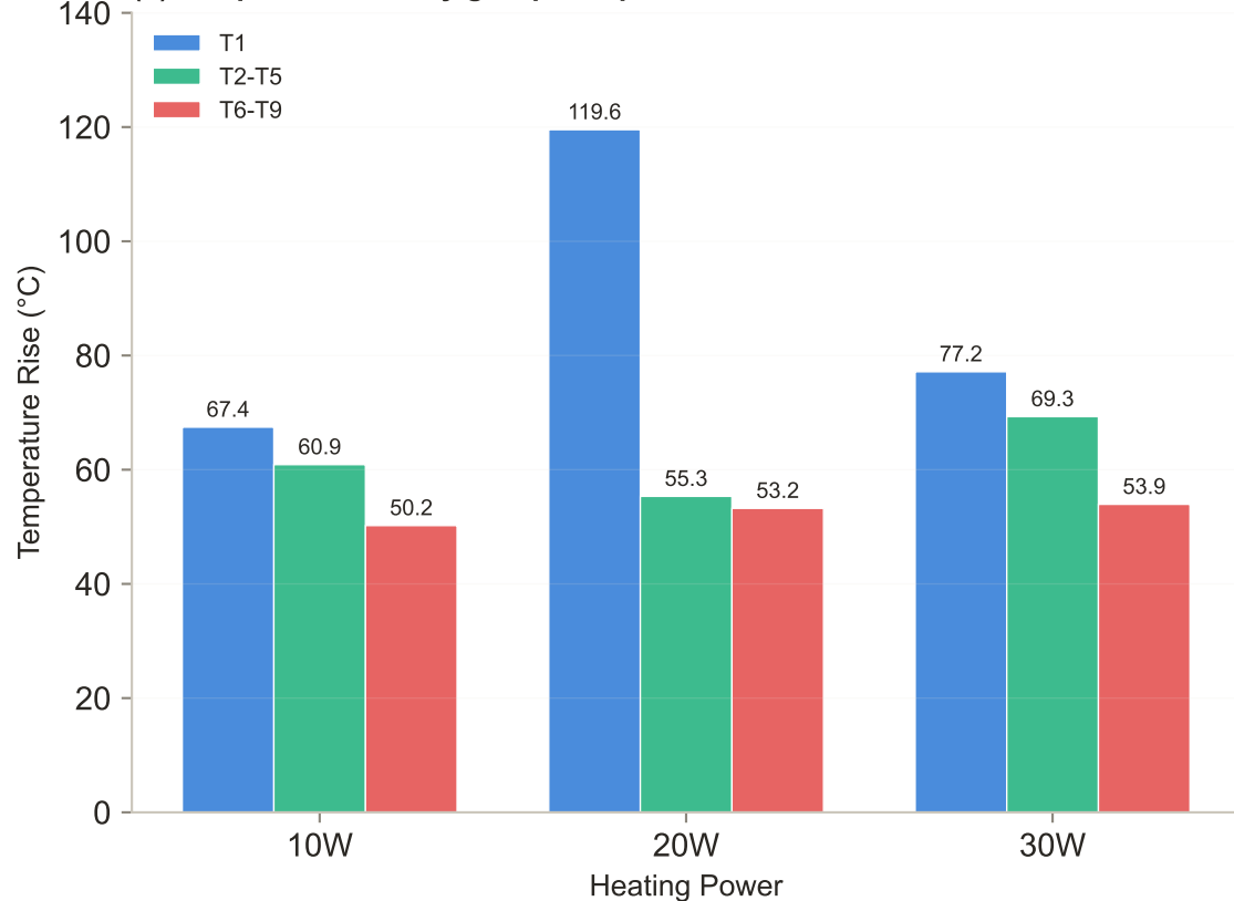
(b) Temperature rise by group and power
