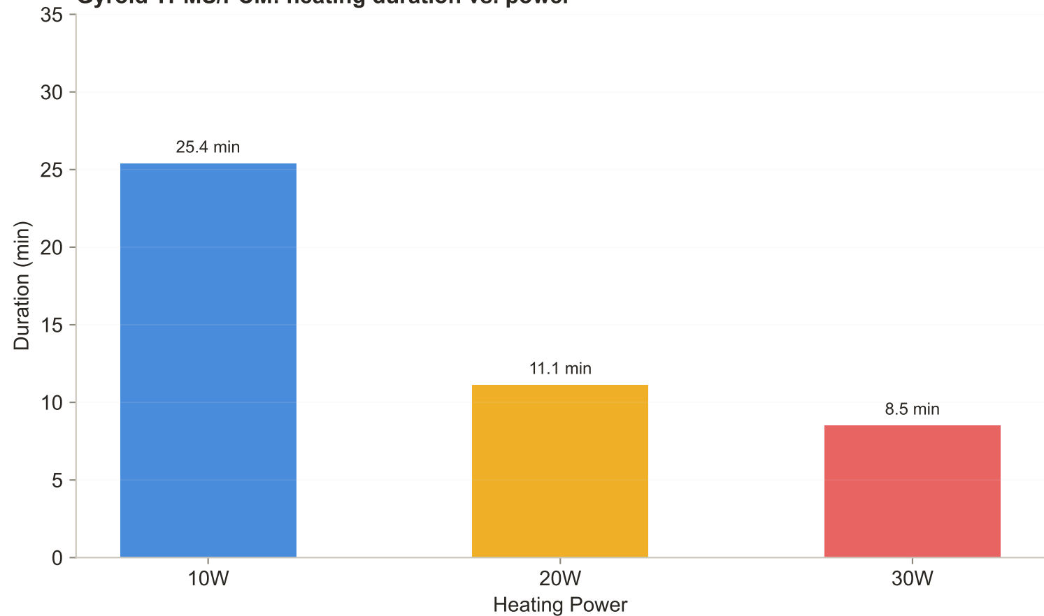
Gyroid TPMS/PCM: heating duration vs. power
