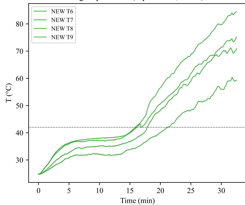
C group sensors (top surface, NEW)
