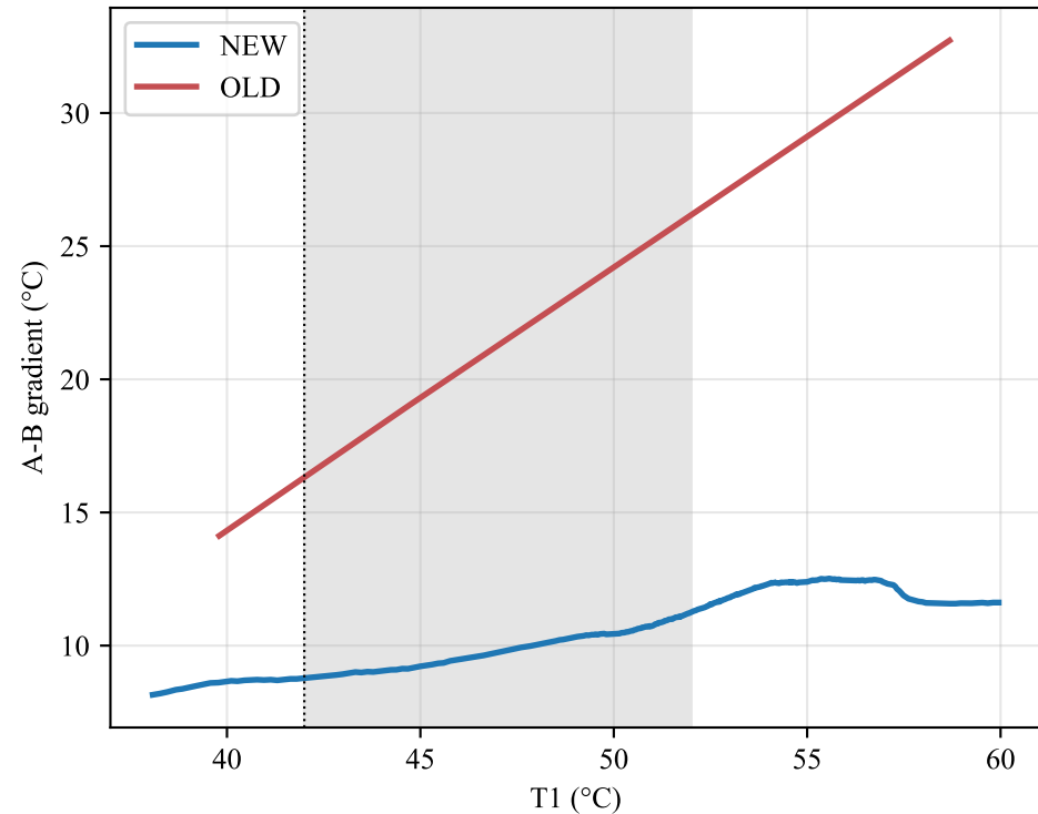
A-B gradient vs T1 (phase-change window shaded)
