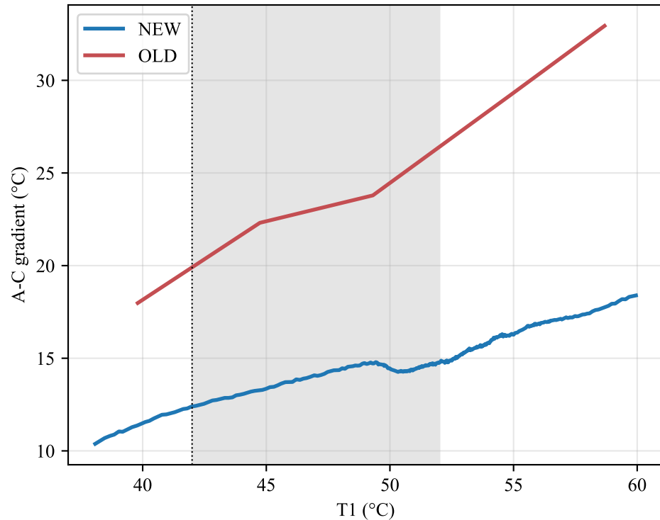
A-C gradient vs T1 (C = T9)
