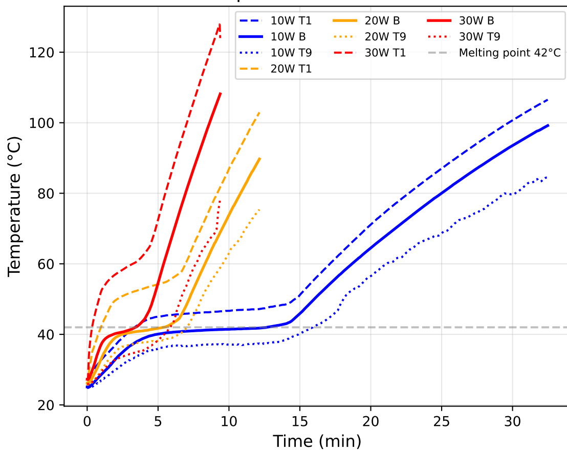
Temperature-time curves
