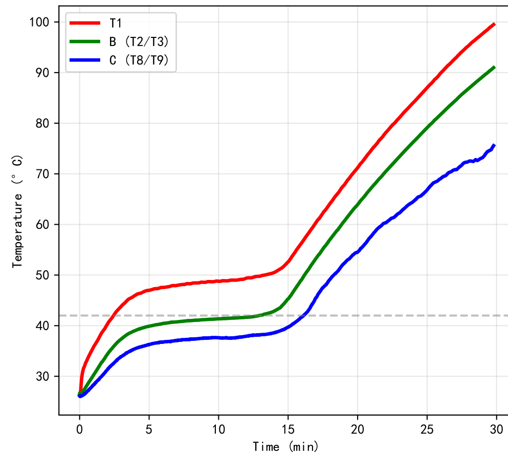
A-C Gradient vs T1 (10W)
