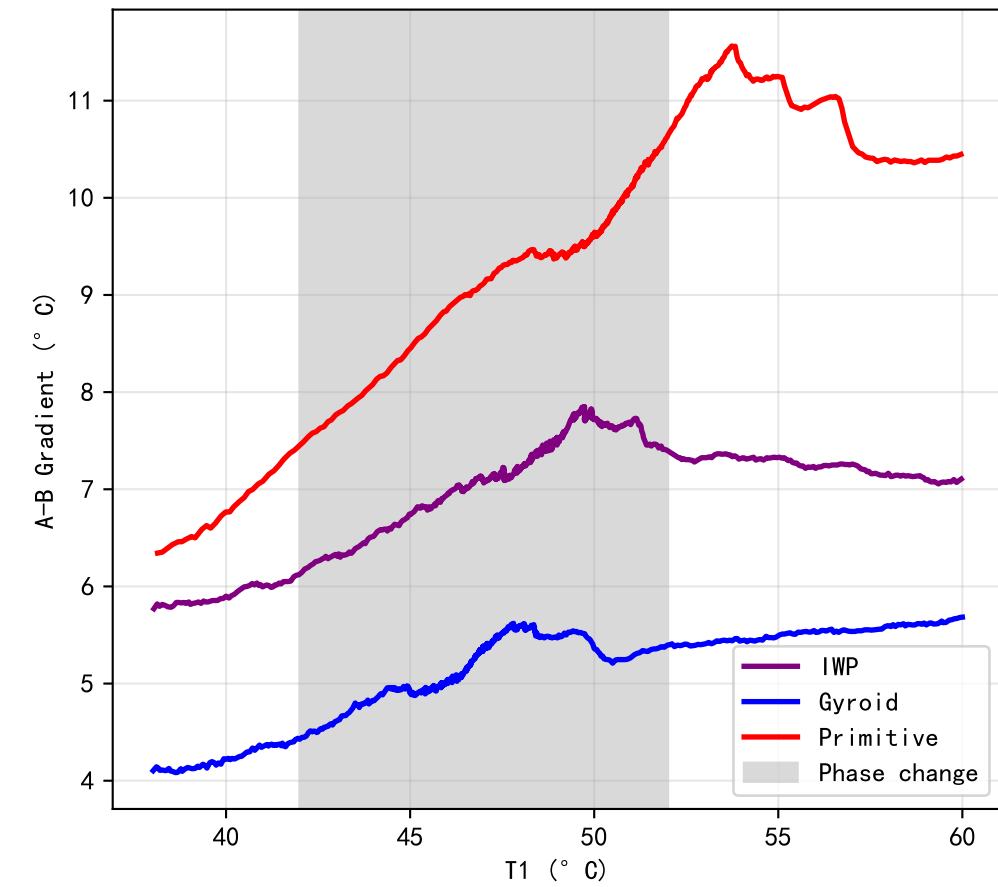
A-B Gradient vs T1 (10W)
