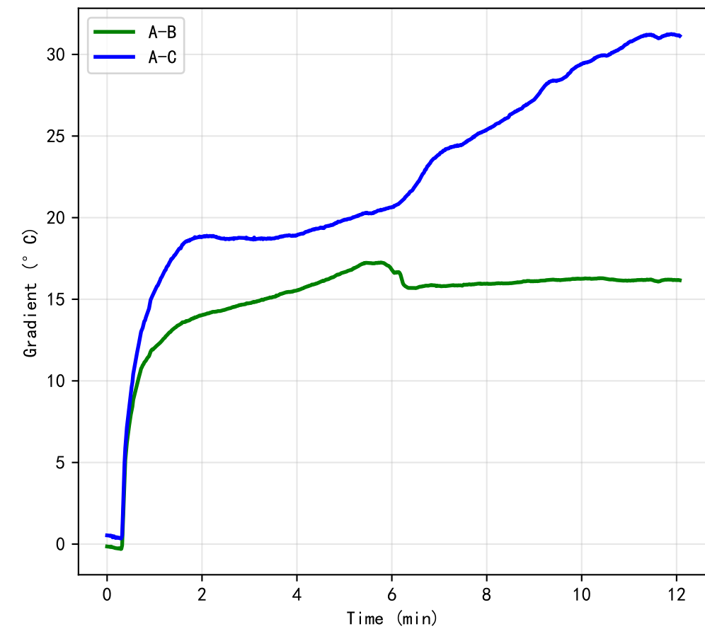
IWP 20W Heating Rate
