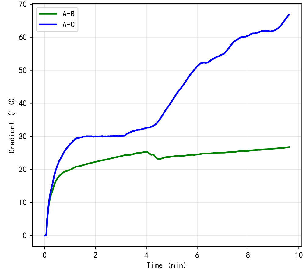
IWP 30W Heating Rate
