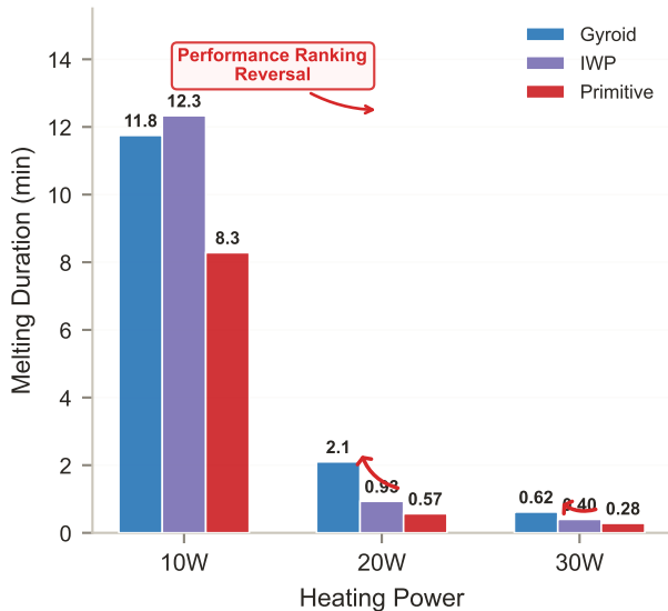
(a) Melting Duration by Structure
