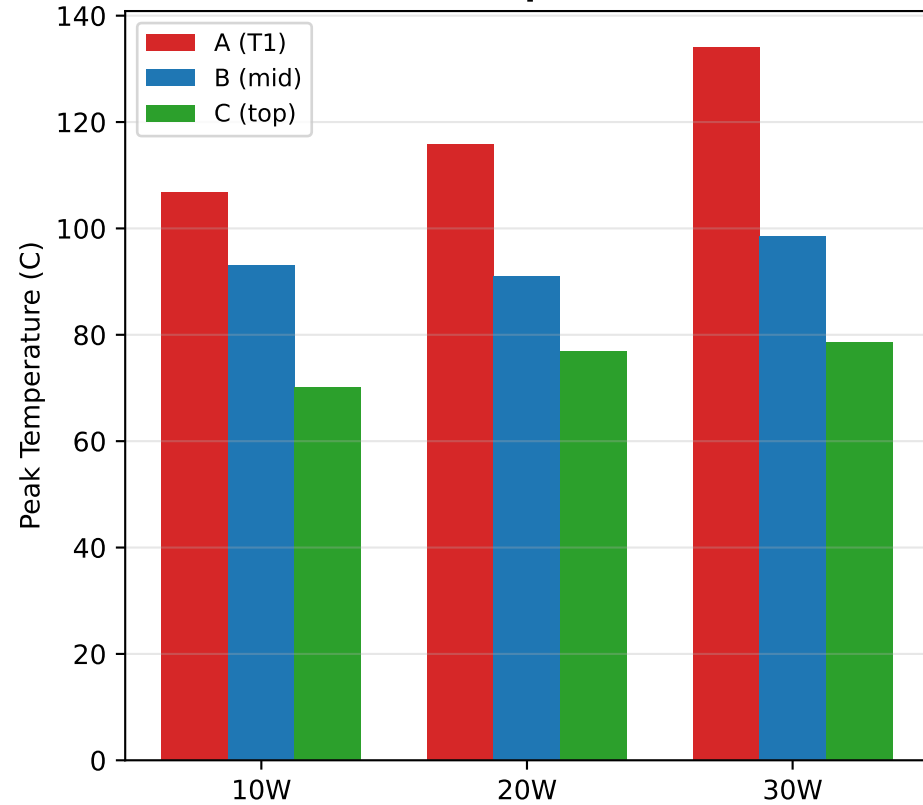
Peak Temperatures
