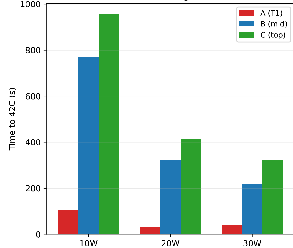
PCM Melting Time
