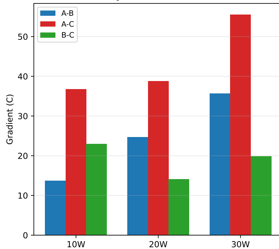
Temperature Gradients
