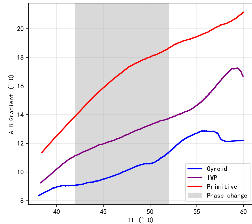
Melting Duration (T1 in 42–52° C, 20W)
