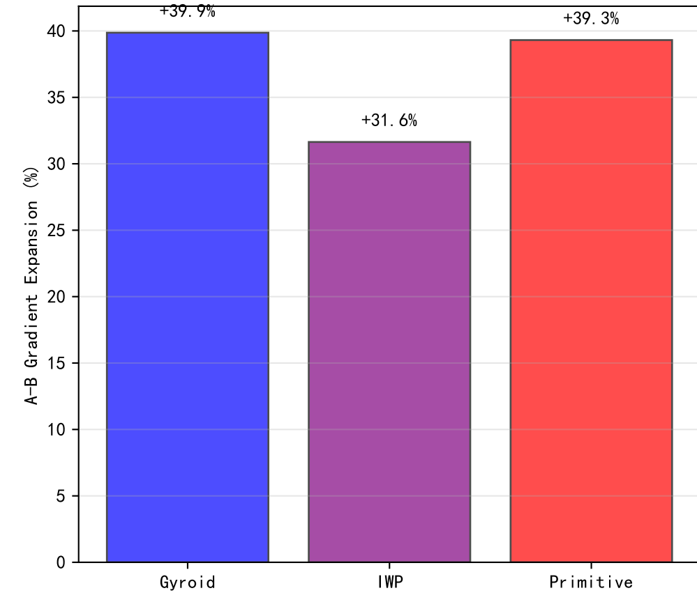
Gradient Expansion Rate (42→55° C, 20W)
