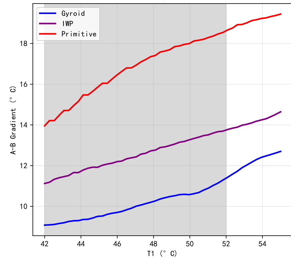
Gradient Expansion Rate (42→55° C, 20W)
