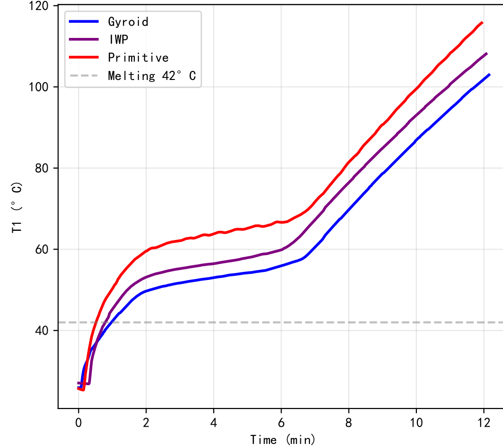
T1 Temperature vs Time (20W)
