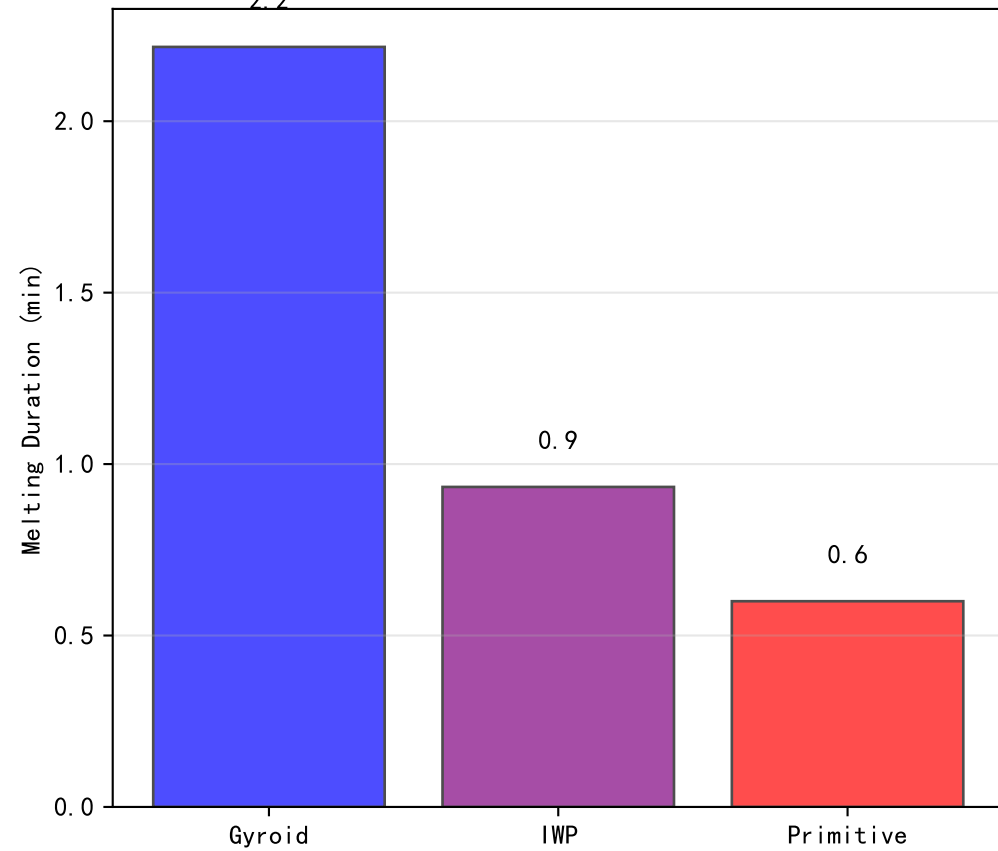
Melting Duration (T1 in 42–52° C, 20W)
