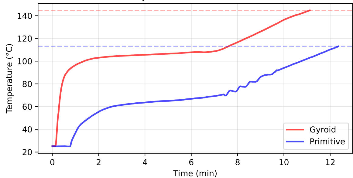
Temperature Gradients Over Time
