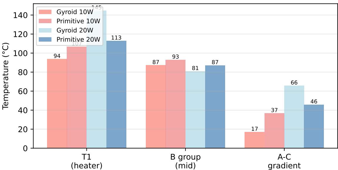
Performance Reversal: 10W vs 20W
