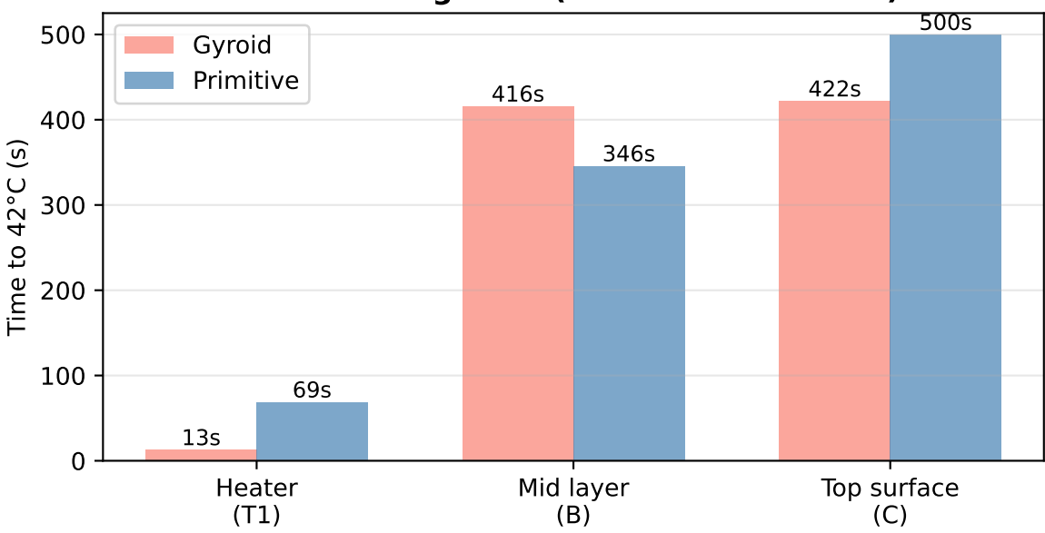
PCM Melting Time (Time to Reach 42°C)
