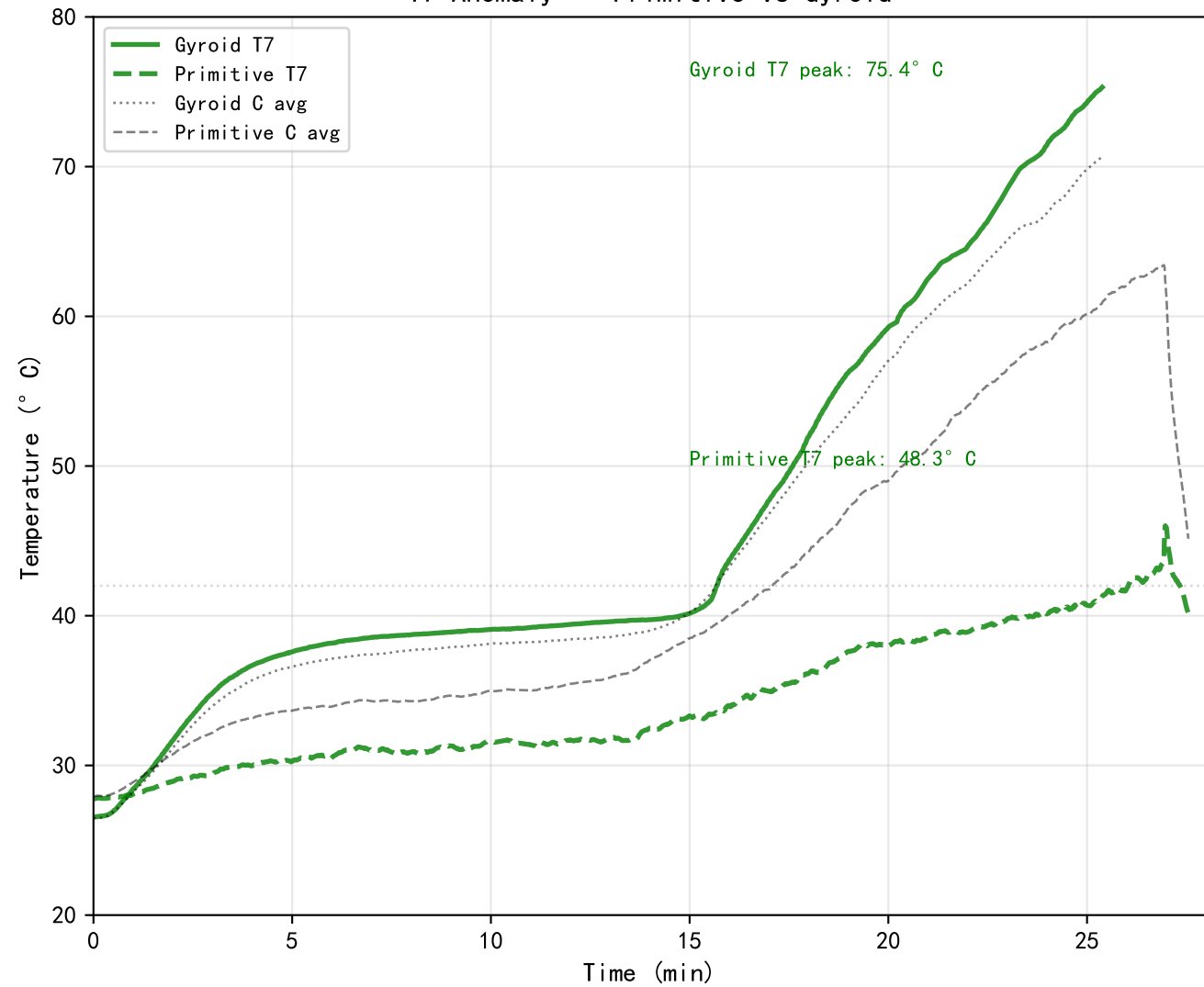
T7 Anomaly — Primitive vs Gyroid
