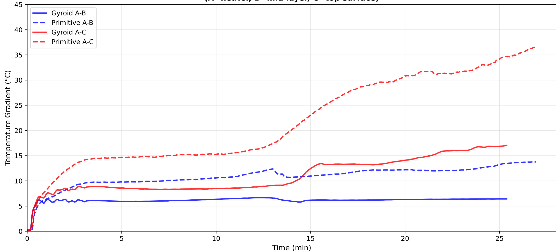
Thermal Gradients — Corrected Statistics (A=heater, B=mid layer, C=top surface)
