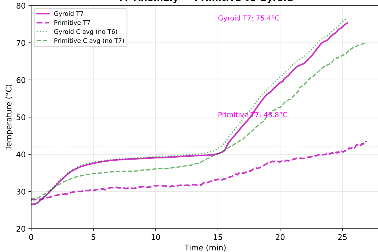
T7 Anomaly — Primitive vs Gyroid
