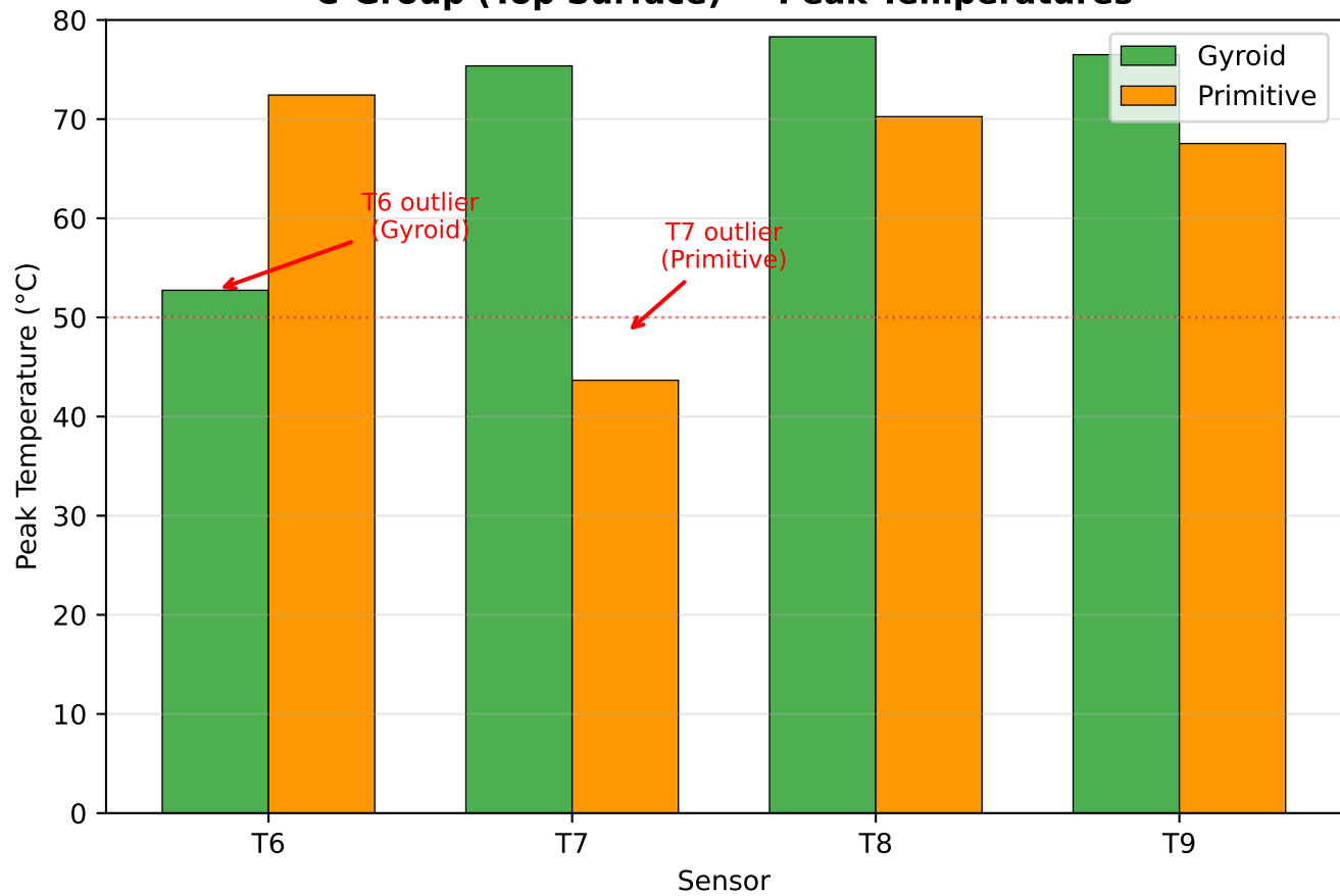
C-Group (Top Surface) — Peak Temperatures
