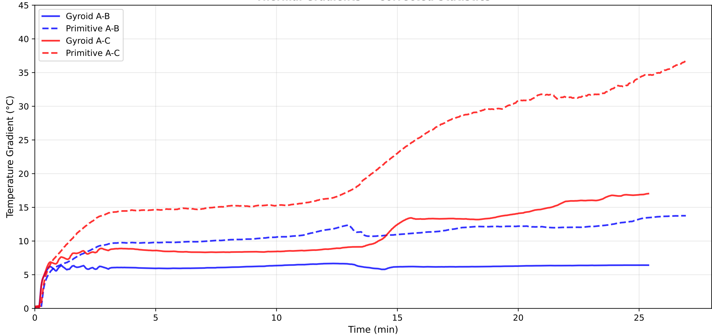
Thermal Gradients — Corrected Statistics
