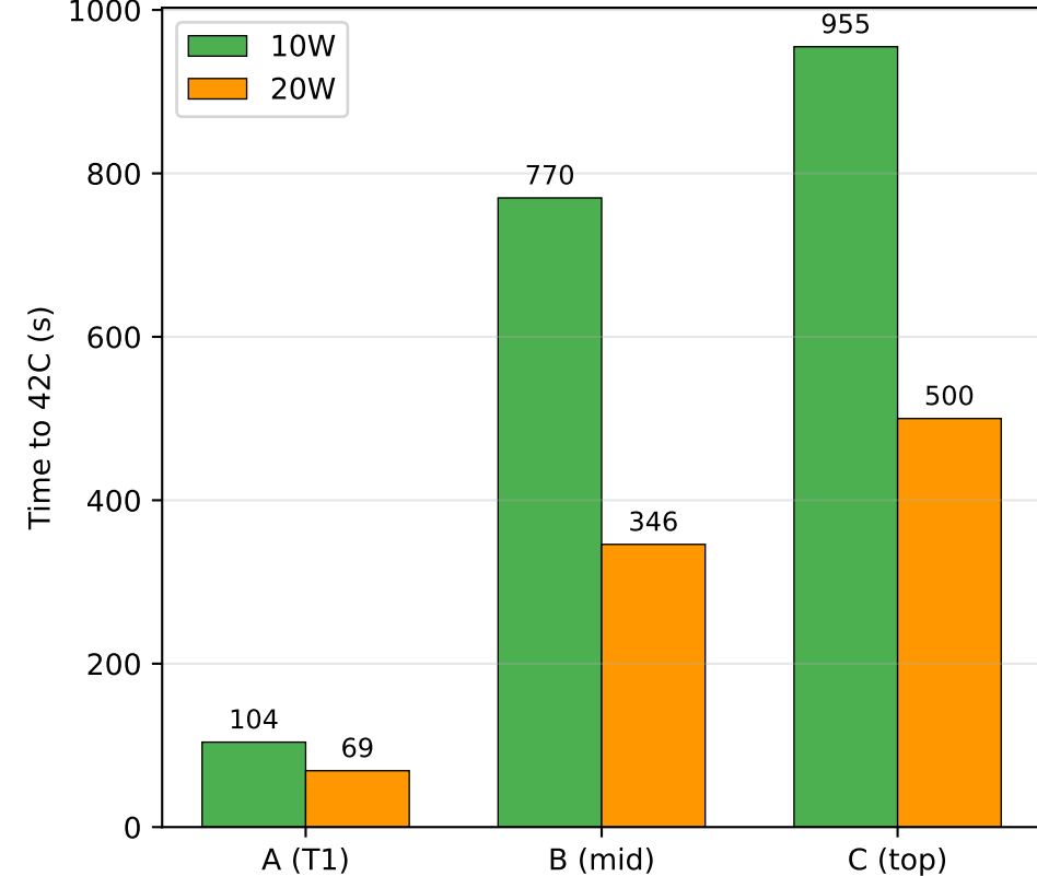
Time to Reach PCM Melting Point
