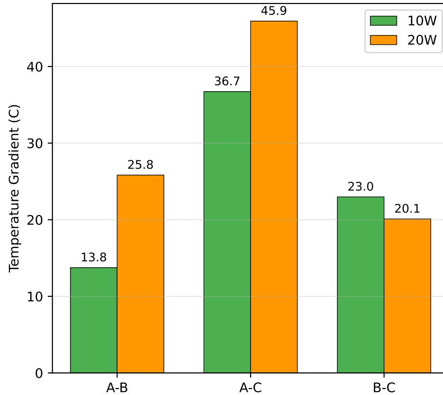
Temperature Gradients at T1 Peak
