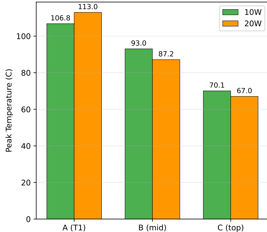
Peak Temperatures by Group
