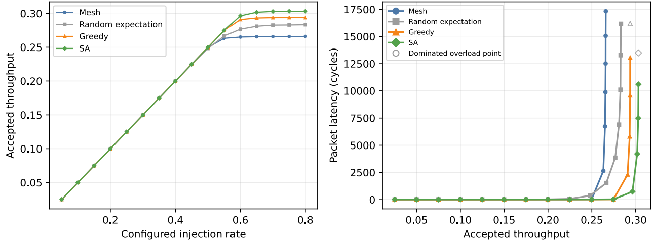
Figure 3: Uniform injection and throughput-latency Pareto curves.
