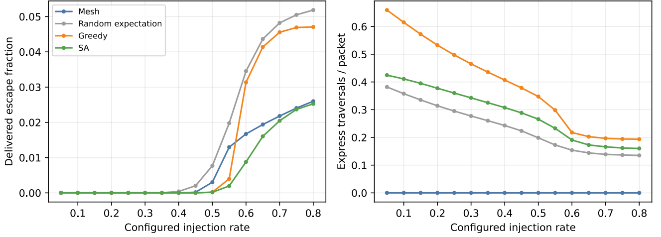
Figure 8: Escape use and express traversals per delivered Uniform packet.
