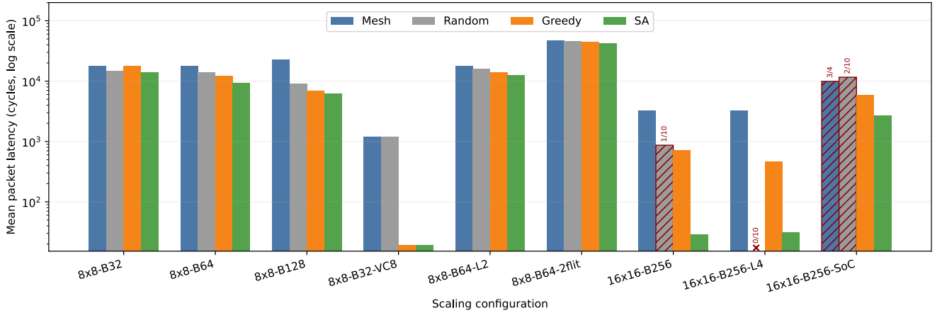
Figure 13: Garnet mean latency for the same configurations (log scale), using the same censoring notation as figure 12.
