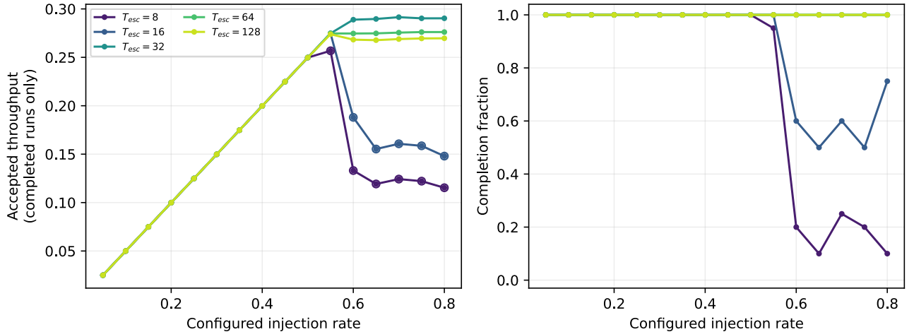
Figure 10: Garnet escape-timeout sensitivity. Throughput is conditional on completion; hollow overlaid markers identify points with censored runs, whose completion fractions are shown at right.
