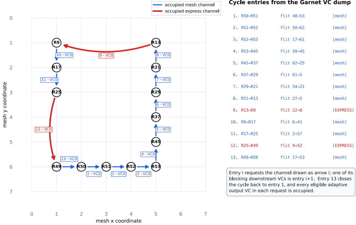
Figure 11: A 13-channel wait-for cycle reconstructed from the Garnet VC dump for escape-off seed 1 at cycle 5655. Numbered arrows show the dependency order; red arcs are express channels and blue arcs are mesh channels.
