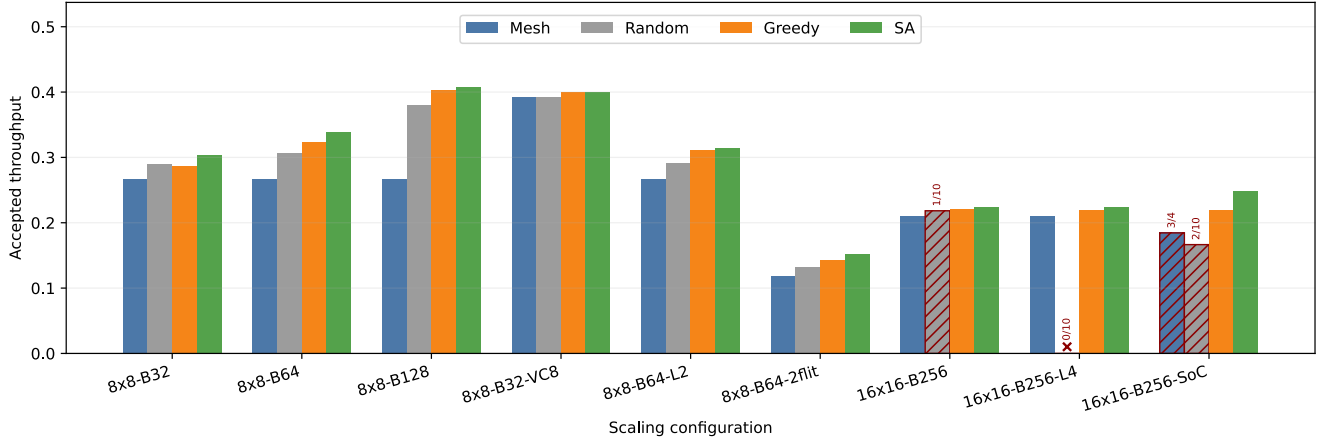
Figure 12: Garnet accepted throughput under the scaling configurations. Hatched bars are conditional means from censored groups; labels give completed/attempted runs, and a crossed marker denotes no valid completed sample. The 8-by-8 rows use one Random layout, whereas the 16-by-16 rows use five.
