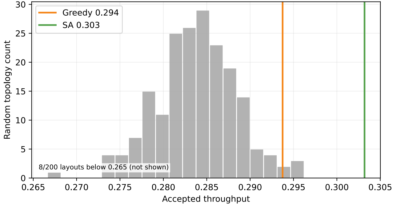
Figure 7: Central Uniform rate-0.8 throughput distribution over 200 random placements; the annotation records layouts below the displayed range.
