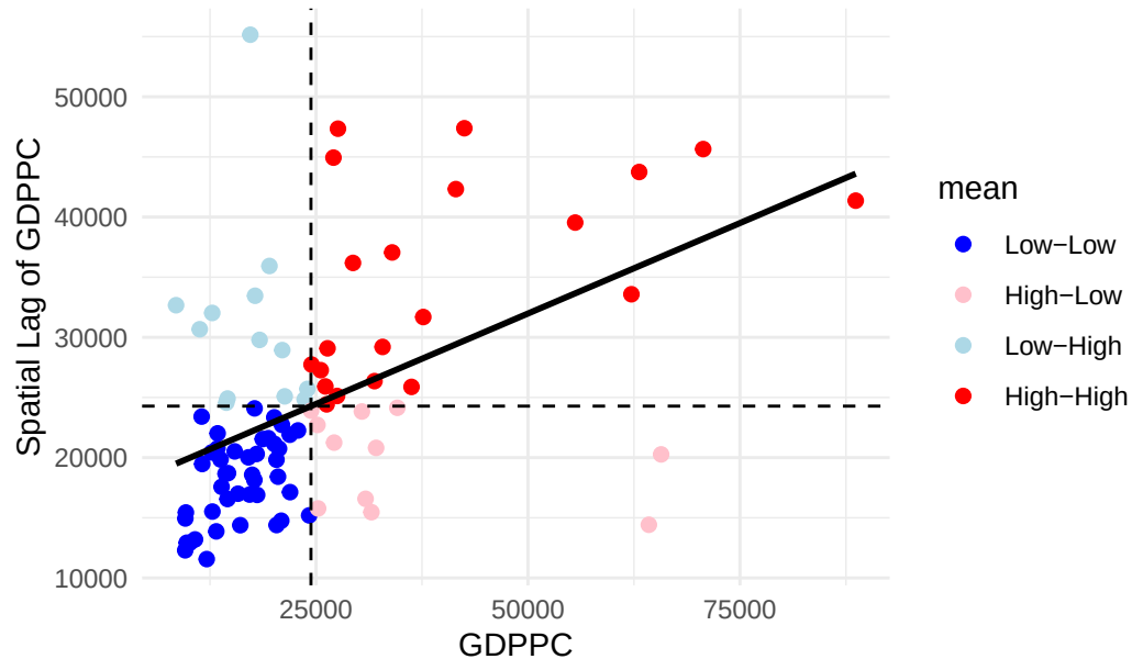
Moran Scatterplot with LISA Quadrants
