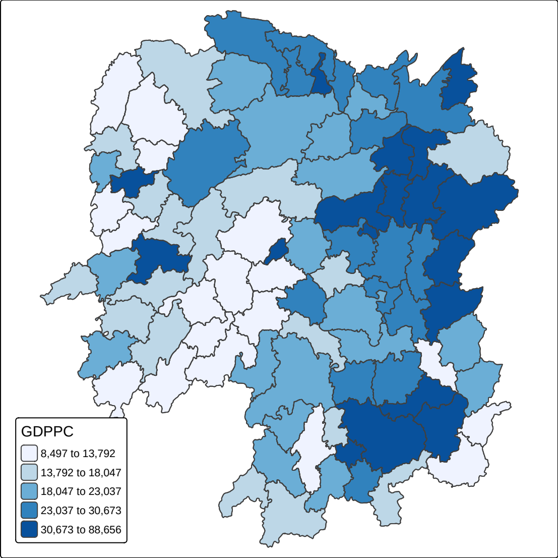
Quantile interval classification
