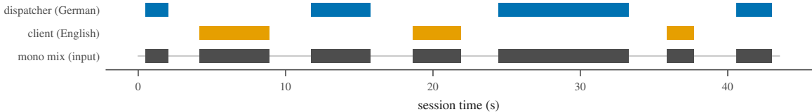
(b) L0 mediated: speaker-change gaps 2.11–2.87 s, session 43.5 s
