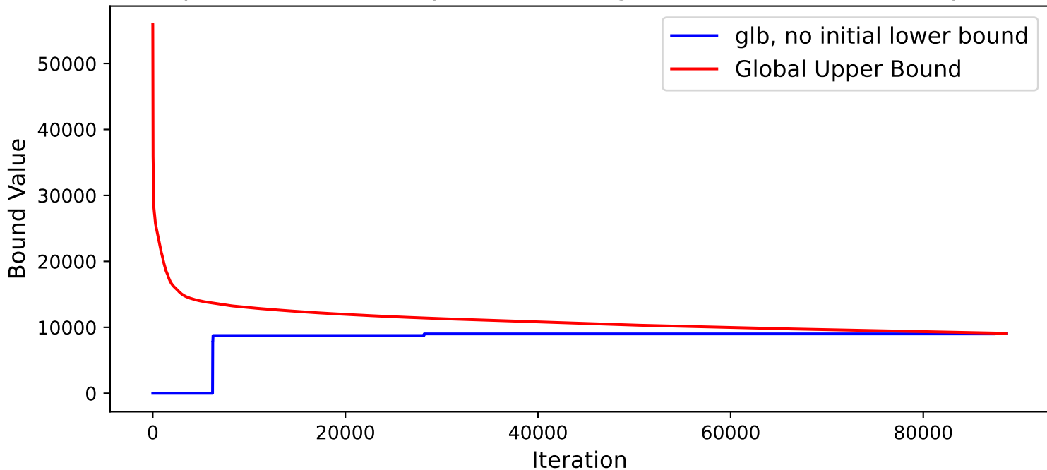
ExLipBaB Bound History (Bike Sharing data,[11,24,24,1], GroupSort)
