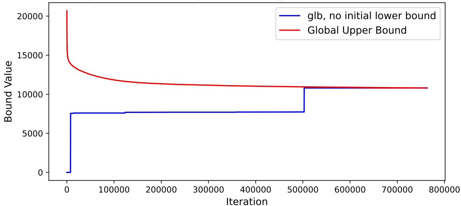
ExLipBaB Bound History (Bike Sharing data,[11,24,24,1], ReLU)
