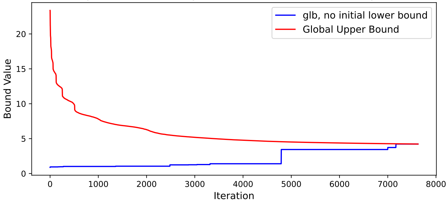
ExLipBaB Bound History (Wine data,[11,24,24,1], GroupSort)
