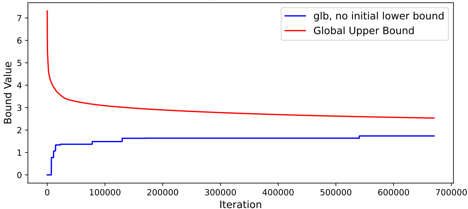
ExLipBaB Bound History (Wine data,[11,24,24,1], ReLU)
