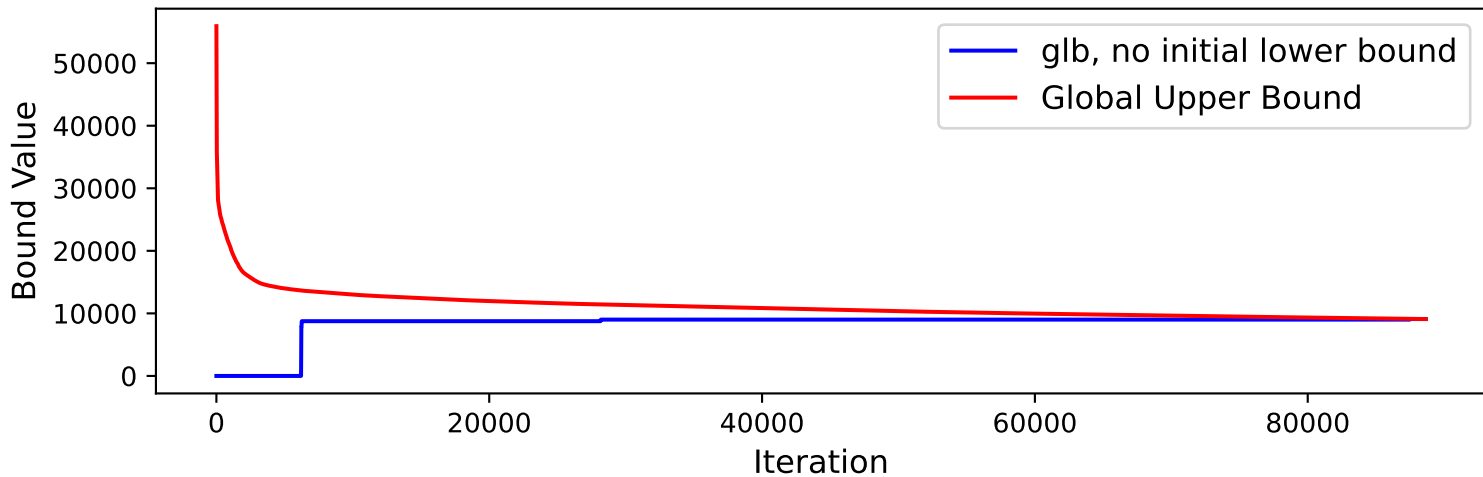
ExLipBaB Bound History (Wine data,[11,12,12,1], ReLU)
