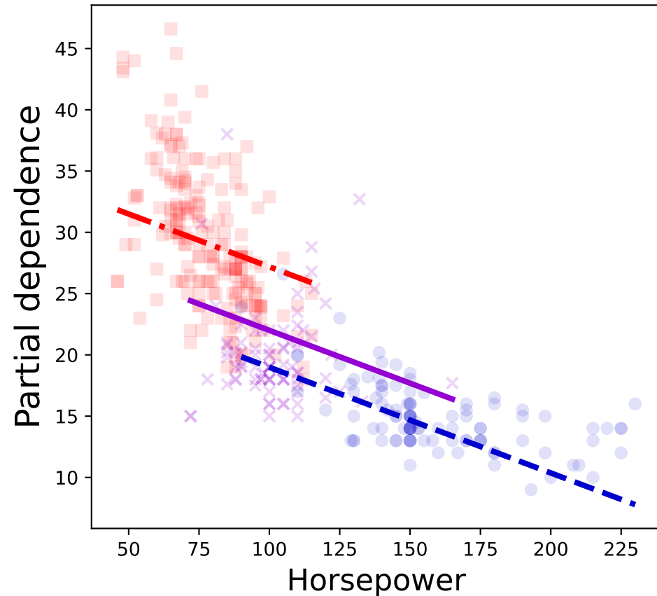
Linear Model
