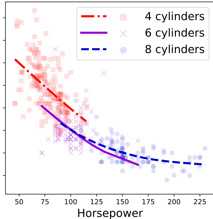
Neural Network
