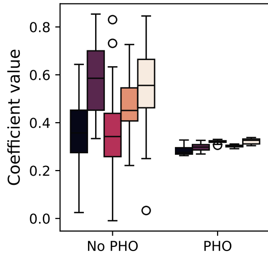
model_year
