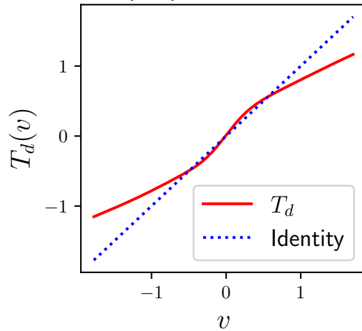
(b.1) T_d : \mathbb{R} \rightarrow \mathbb{R}
