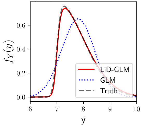
(a.2) Density for fixed \mathbf{x}
