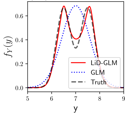
(b.2) Density for fixed \mathbf{x}
