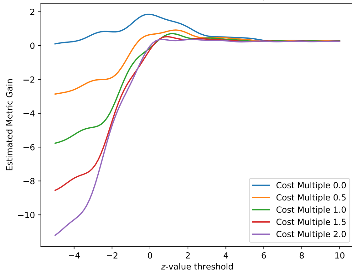
Return Curves under Cost Multipliers
