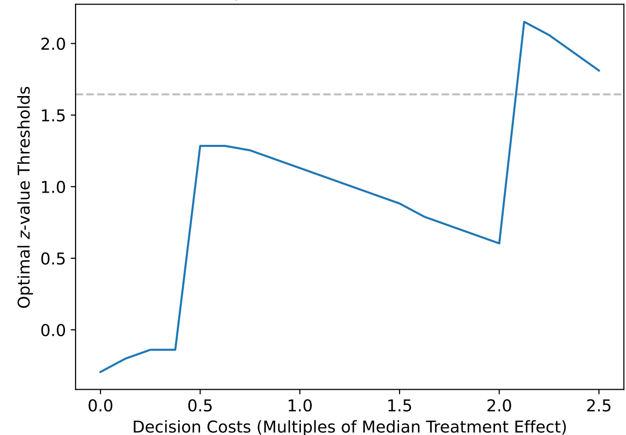
Optimal Threshold vs. Cost
