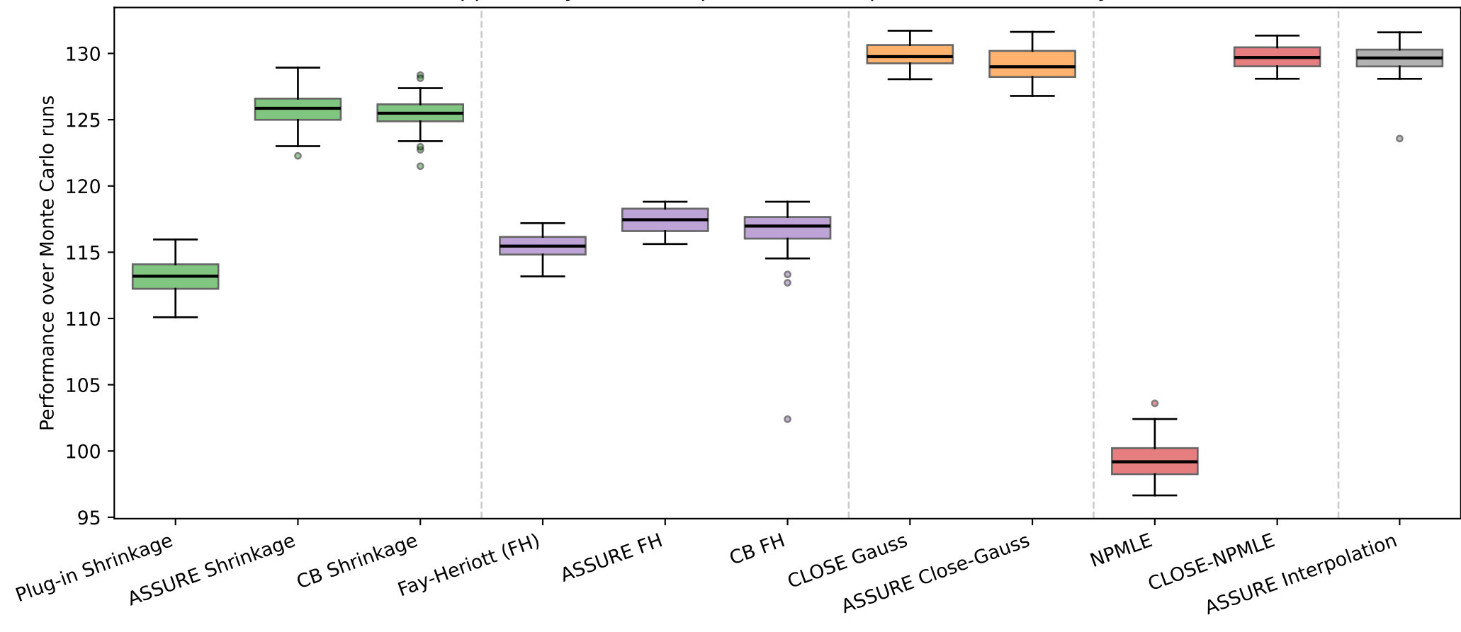
Opportunity Atlas Comparison: Well-Specified Model, Noisy X
