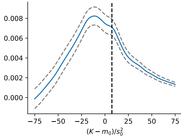
Cost = 0.369 ~ (Naive chooses 1/3)
