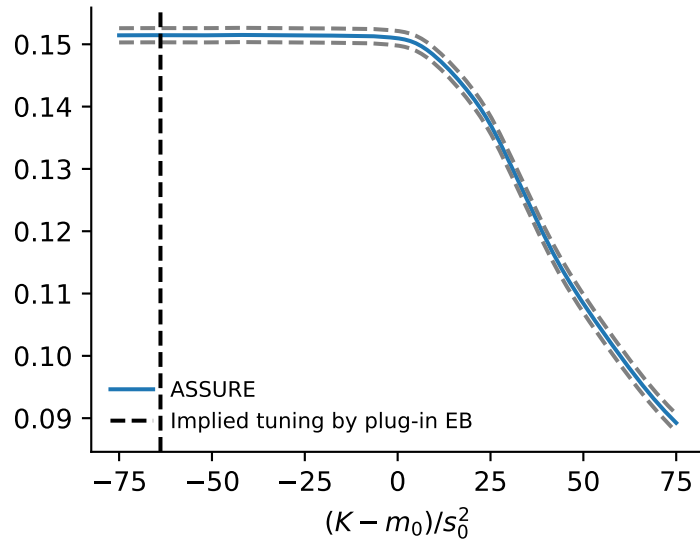
Cost = 0.2 ~ (Improving on status quo)
