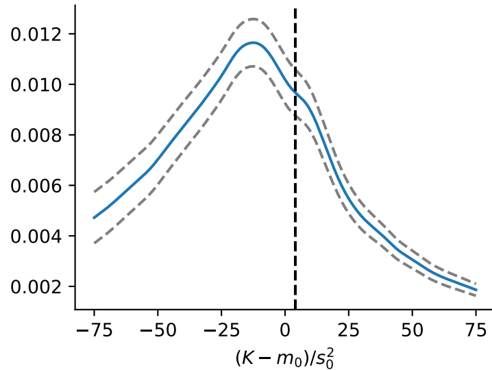
Cost = 0.361 ~ (Plug-in EB chooses 1/3)
